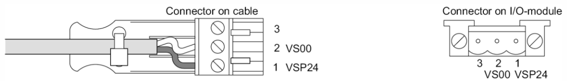
Figure 50 24V Power input
