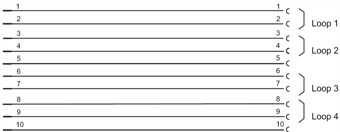
Figure 51 Layout flatcable
